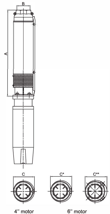
4" motor
